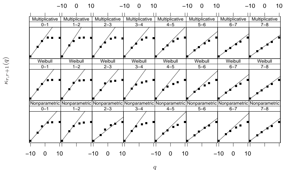
FIG 9. Moment-statistic m -slopeplot for one Auckland trace.
