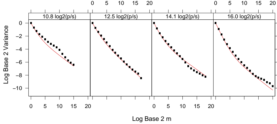
FIG 16. Four variance rate-time plots for 4 Auckland trace segments. The log model variance, \log_2 V_{\bar{z}_v^{(m)}} (—), and the log nonparametric variance, \log_2 \hat{V}_{\bar{z}_v^{(m)}} (●), are graphed against \log_2 m .
