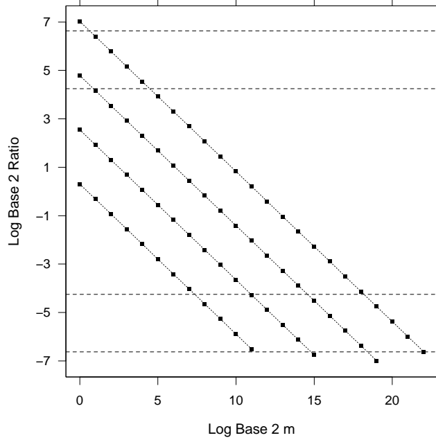
FIG 18. \zeta(\alpha, m) is plotted against \log_2(m) for each of four values of \log_2(\alpha) : 10.5, 13.5, 16.5, and 19.5 log base 2 p/s. The points for each value of \log_2(\alpha) lie on a line; the intercepts of the lines increase with \log_2(\alpha) . The horizontal dashed lines show values of \zeta(\alpha, m) for which the percentages of the variances of the white noise term are, from top to bottom, 99%, 95%, 5%, and 1%.
