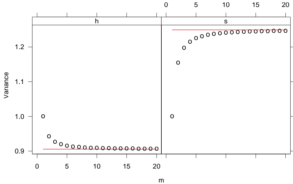
FIG 14. Plotted against m for d = 0.31 are V_{\tilde{h}_v^{(m)}}/\sigma_h^2 ( \circ ) and \tilde{V}_{\tilde{h}_v^{(m)}}/\sigma_h^2 ( - ) in the left panel, and V_{\tilde{s}_v^{(m)}} ( \circ ) and \tilde{V}_{\tilde{s}_v^{(m)}} ( - ) in the right panel.
