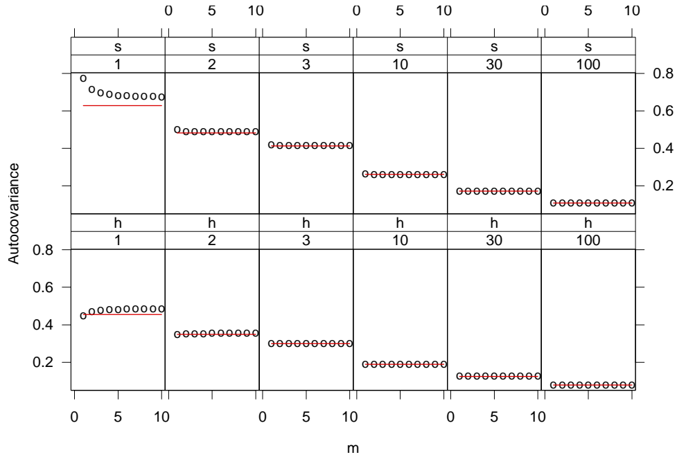
FIG 15. Each panel plots true ( \circ ) and approximate ( — ) autocovariances against m for the scaled sum shown in the top strip label of the panel ( h for h_u , and s for s_u ) and for the lag shown in the lower strip label.
