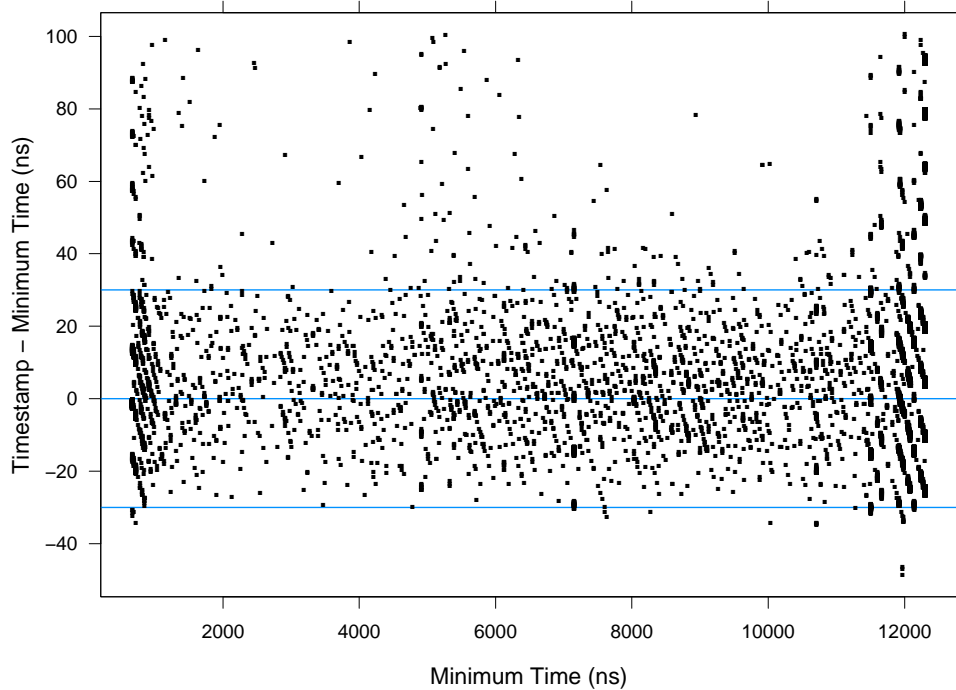
FIG 1. Accuracy and delay-identification plot for one live Auckland 15-minute trace segment.
