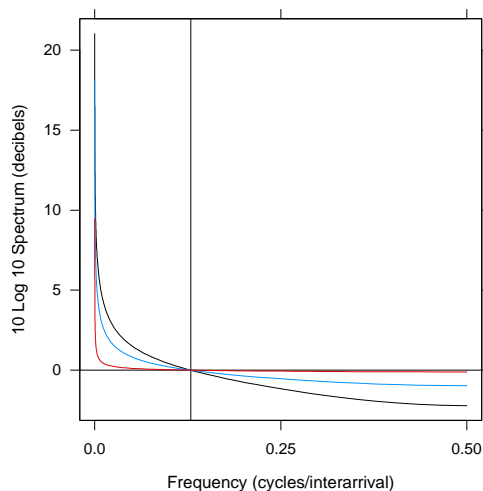
FIG 5. Log power spectra \ell_z(f) for d = 0.31 and 3 values of \theta .
