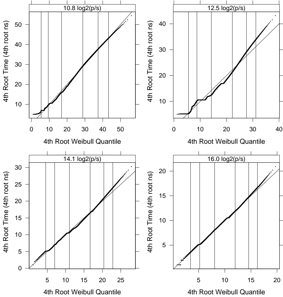
FIG 3. Weibull quantile plots of interarrivals of 4 Auckland trace segments.
