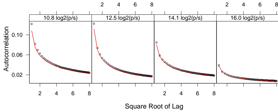
FIG 20. Power series approximation (—) of multiplicative MFSD autocorrelations (○).
