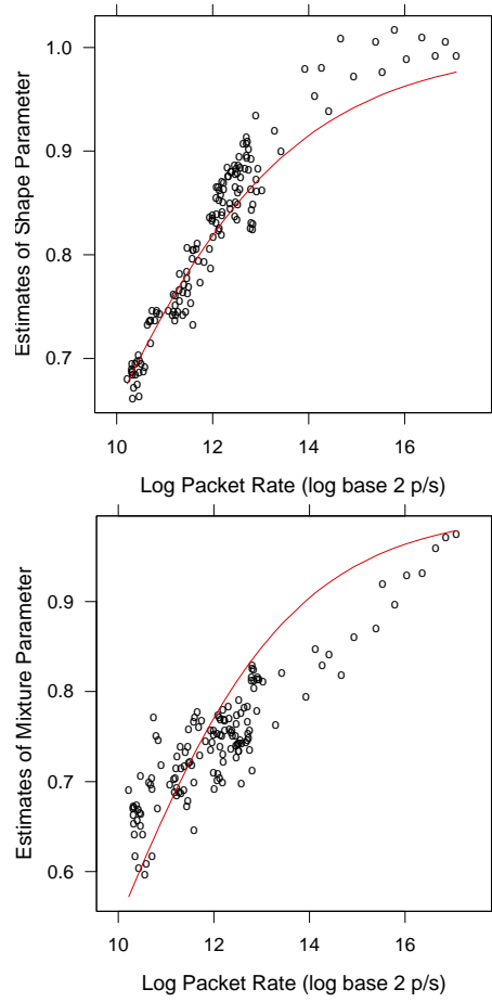
FIG 11. \hat{\lambda}_k (upper panel \circ ) and \hat{\theta}_k (lower panel \circ ) are plotted against \log_2(\hat{\alpha}_k) . Derived equations \lambda(\alpha) (upper panel \text{—} ) and \theta(\alpha) (lower panel \text{—} ) are plotted against against \log_2(\alpha) .
