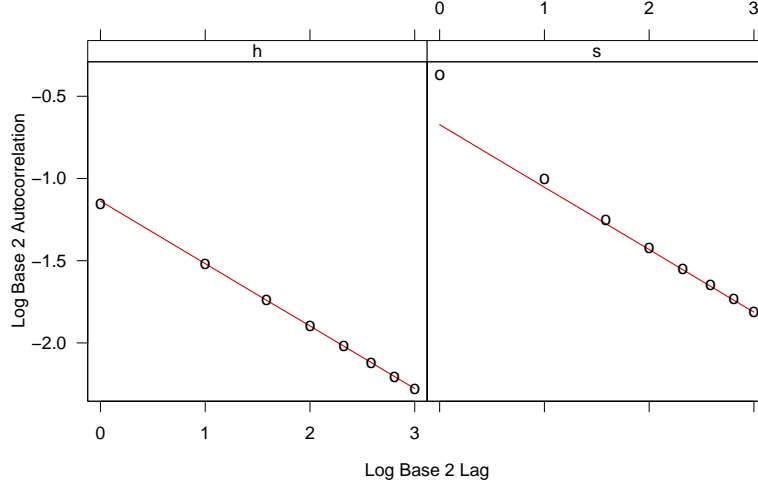
FIG 13. Log base 2 autocorrelation with d = 0.31 vs. log base 2 lag. Left: \rho_h(k) ( \circ ), \check{\rho}_h(k) ( — ). Right: \rho_s(k) ( \circ ), \check{\rho}_s(k) ( — ).
