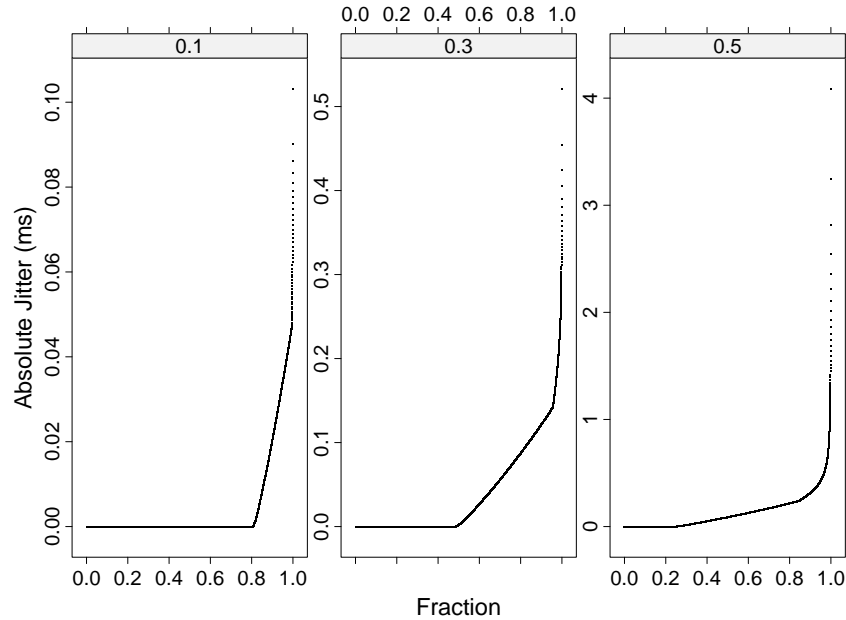
FIG 24. Quantiles of Absolute Jitter
