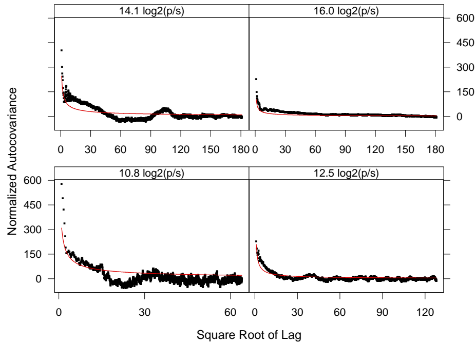
FIG 22. For m = 128 , normalized nonparametric estimates of autocovariances ( \bullet ), and normalized approximate autocovariances ( \text{---} ) for t_v^{(m)} are plotted against \sqrt{k} for the 4 Auckland trace segments.
