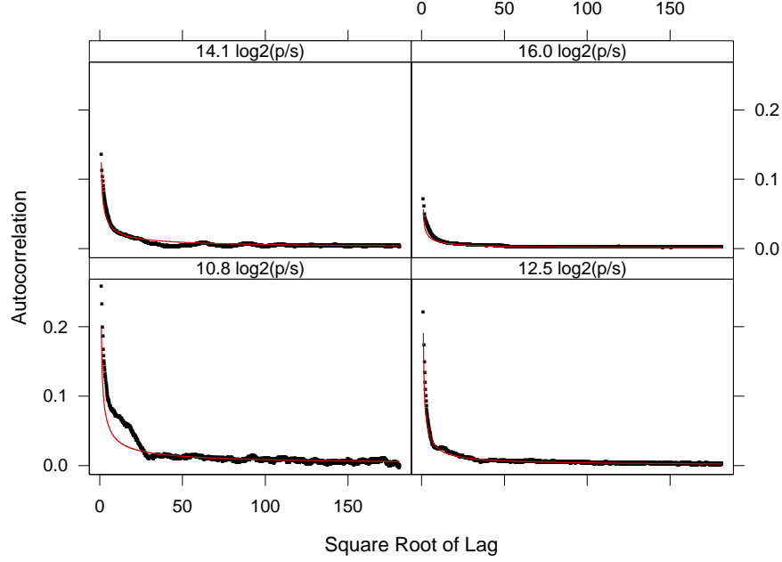
FIG 12. Nonparametric estimates (●) and GFSD model estimates (—) of autocorrelation are plotted against square root lag for 4 Auckland trace segments.
