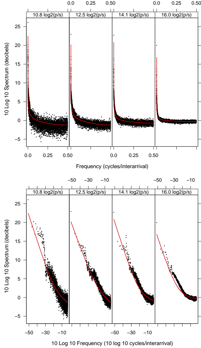
FIG 7. 10 \log_{10}(\bar{I}(\bar{f}_j)) ( \bullet ) and 10 \log_{10}(\hat{p}_z(\bar{f}_j)) ( \rightarrow ) for 4 trace segments.
