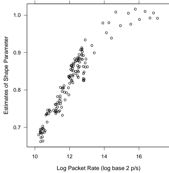
FIG 4. \hat{\lambda}_k is plotted against \log_2(\hat{\alpha}_k) for the 144 Auckland trace segments.
