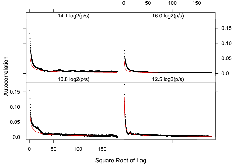
FIG 19. Nonparametric estimates of autocorrelation (●) and estimates from fitted multiplicative MFSD models (—).
