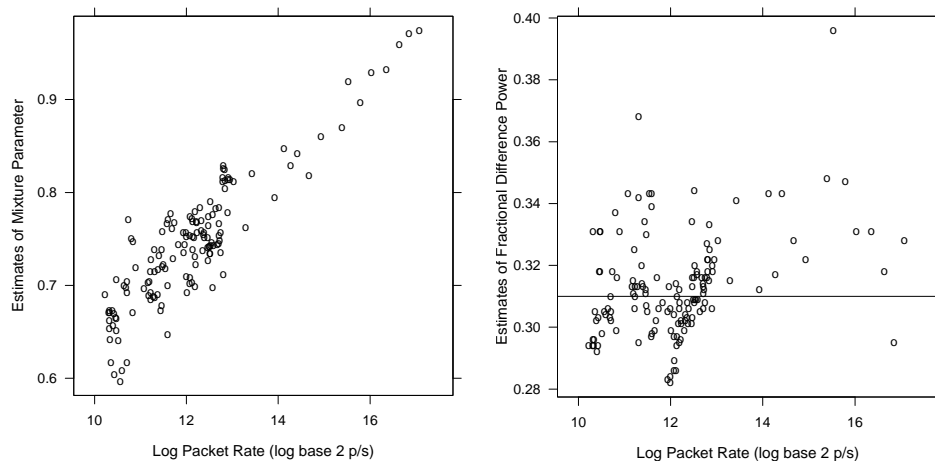
FIG 6. Estimates of the GFSD mixture coefficient \theta and fractional exponent d for the 144 Auckland traces. \hat{\theta}_k (left panel) and \hat{d}_k (right panel) are plotted against \log_2(\hat{\alpha}_k) , the log base 2 estimates of the packet rates. The horizontal line in the right panel show the median, 0.31, of the \hat{d}_k .
