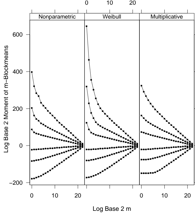
FIG 8. Moment-statistic m -plot for one Auckland trace.
