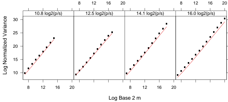
FIG 21. The log base 2 of normalized nonparametric estimates of variances ( \bullet ), and the log base 2 of normalized approximate variances ( \text{---} ) for t_v^{(m)} , are plotted against \log_2(m) for the 4 Auckland trace segments.
