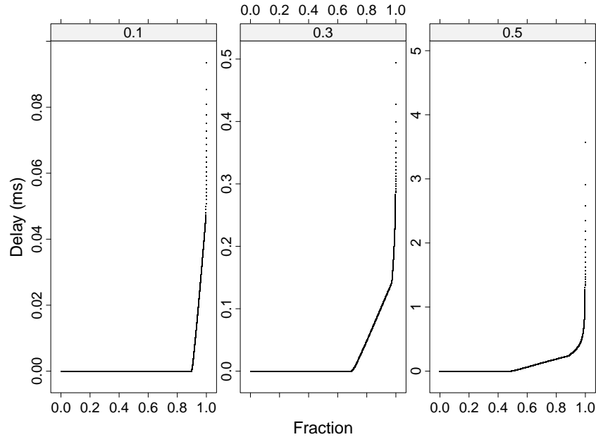
FIG 23. Quantiles of Delay
