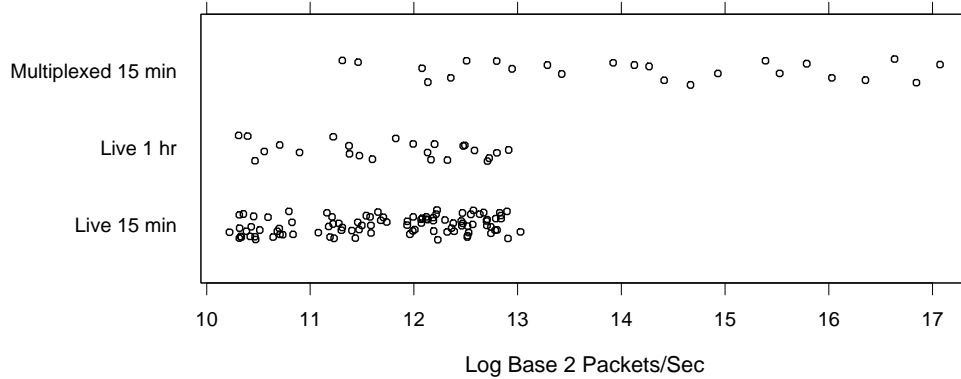
FIG 2. Log base 2 observed packet rates of 144 Auckland trace segments.
